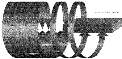
The helical/spiral CT scan speed is synchronized with the conveyor belt speed for complete bag coverage and no gaps in the 3-D image data coverage.
